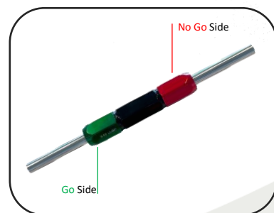
DORO® Skull Pin Limit Gauge
